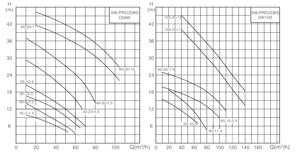
Performance cruve
