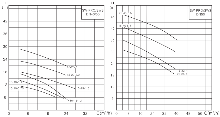
Performance cruve
