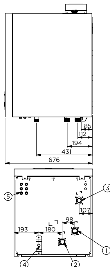
Viwa S 150 Bottom and Side View Measurements
