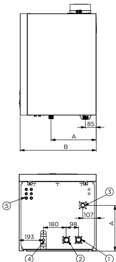
Viwa S 90-125 Bottom and Side View Measurements
